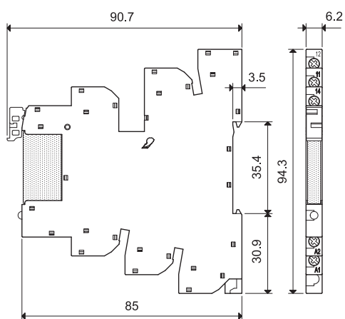
39.80 39.81 Screw terminal
