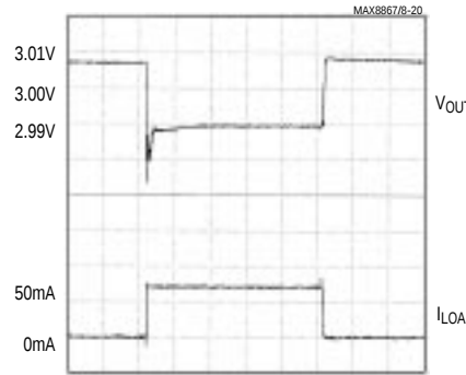
LOAD-TRANSIENT RESPONSE NEAR DROPOUT
