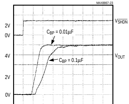
MAX886_EUK50 SHUTDOWN EXIT DELAY
