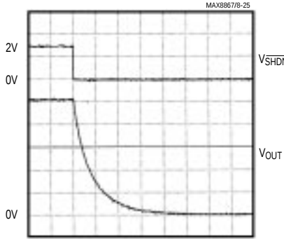
MAX8868 ENTERING SHUTDOWN
