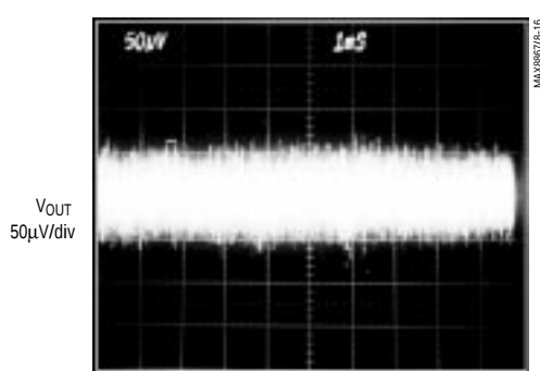
MAX886_EUK25 10Hz TO 100kHz OUTPUT NOISE
