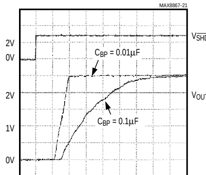
MAX886_EUK25 SHUTDOWN EXIT DELAY
