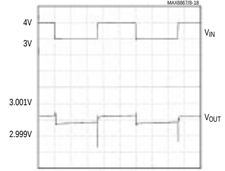
LINE-TRANSIENT RESPONSE
