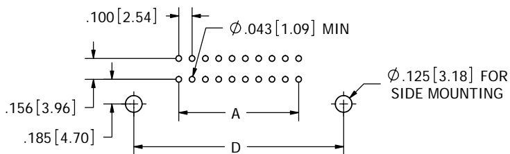
PCB LAYOUT
