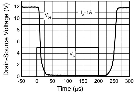
Switching Speed
