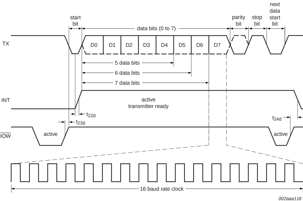
Fig 13. Transmit timing
