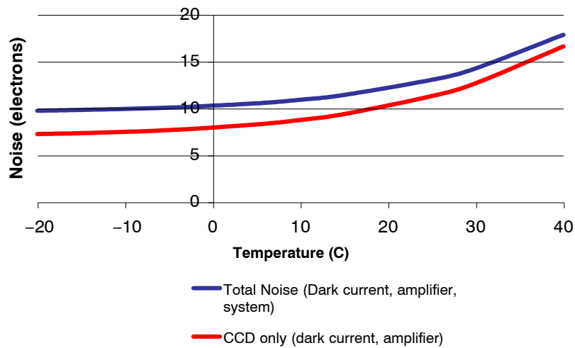
Figure 9. Noise Floor
