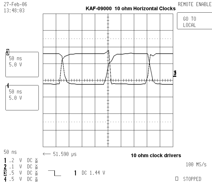
Figure 18. Horizontal Clocks
