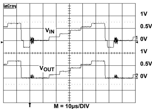
FIGURE 29. VIDEO SIGNAL
