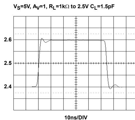
FIGURE 22. SMALL SIGNAL TRANSIENT RESPONSE
