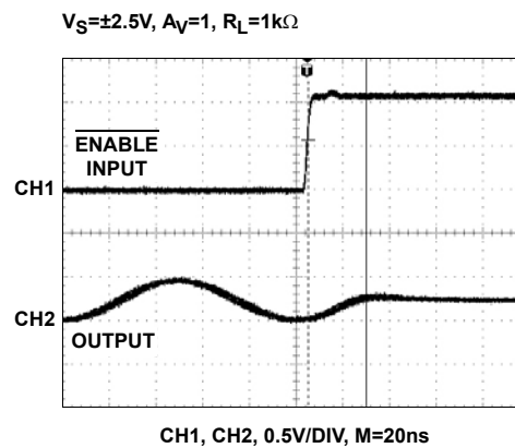
FIGURE 24. DISABLED RESPONSE
