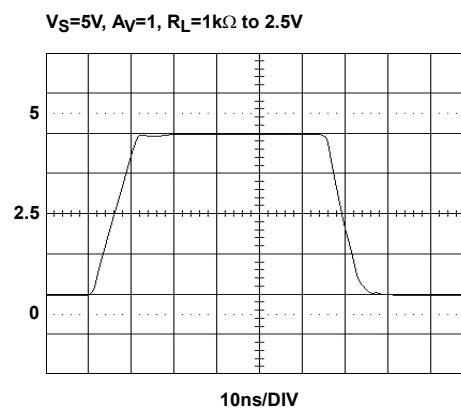
FIGURE 20. LARGE SIGNAL TRANSIENT RESPONSE
