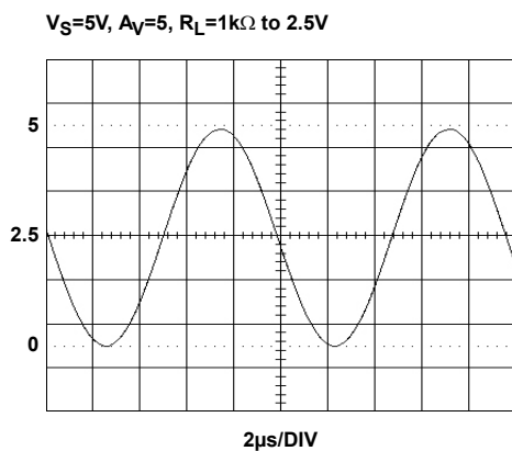
FIGURE 23. OUTPUT SWING
