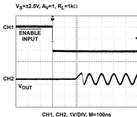
FIGURE 25. ENABLED RESPONSE
