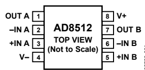
Figure 3. 8-Lead MSOP (RM Suffix)
