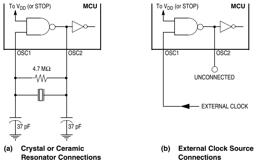
Figure 1-2. Oscillator Connections
