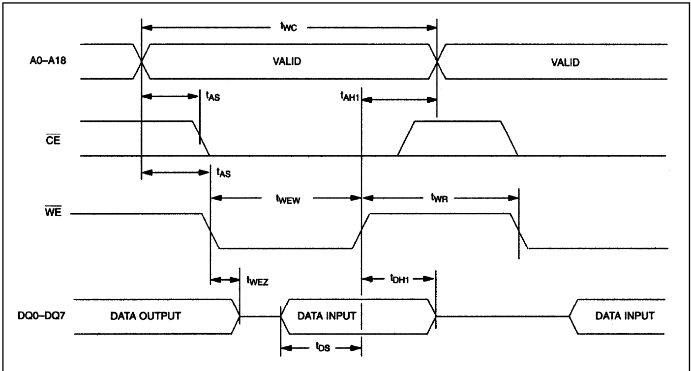
Figure 6. Write Cycle Timing, Write-Enable Controlled
