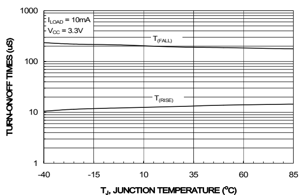
Figure 15. T_{RISE}/T_{FALL} vs. Temperature
