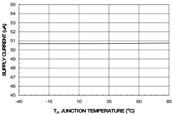
Figure 7. I_{LATCH-OFF} Current vs. Temperature
