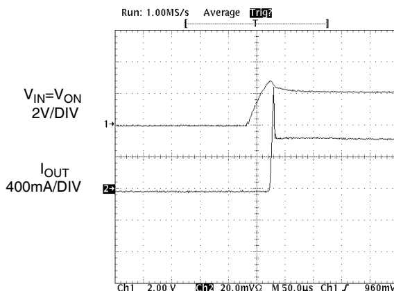
Figure 23. Current Limit Response Time (Switch power up to hard short)
