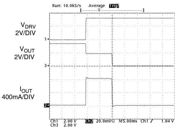
Figure 18. T_{BLANK} Response
