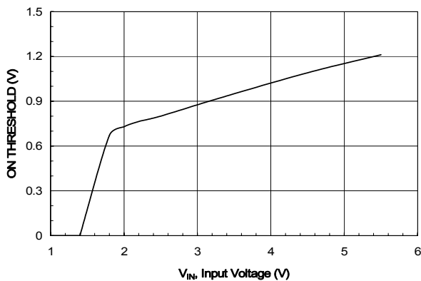
Figure 11. V_{IH} vs. V_{IN}
