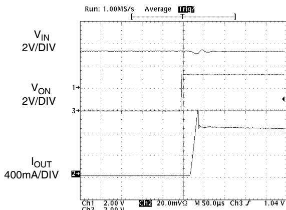
Figure 24. Current Limit Response Time (Output Shorted to GND by 2.2Ω, moderate short)
