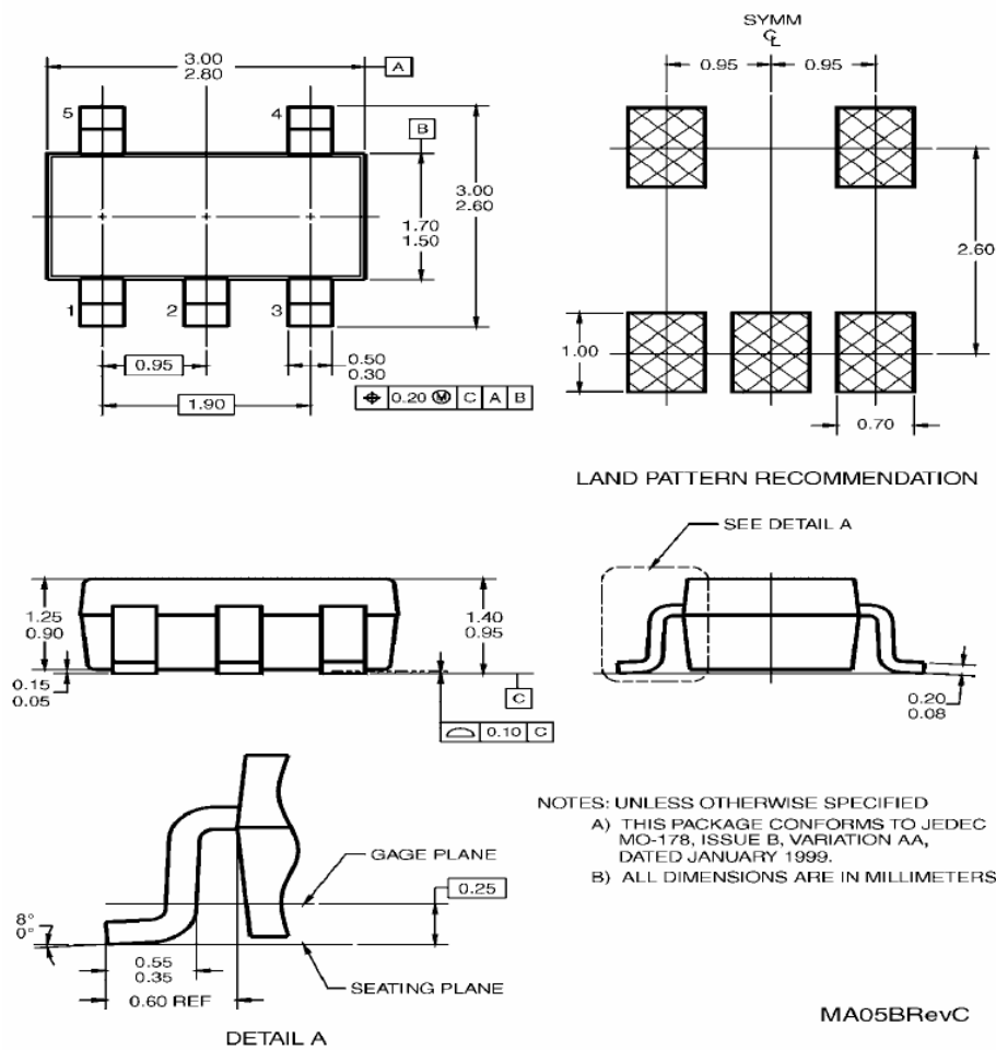
DETAIL A
