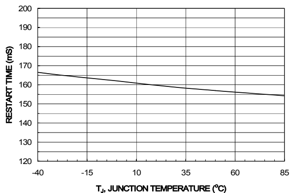
Figure 17. T_{RESTART} vs. Temperature
