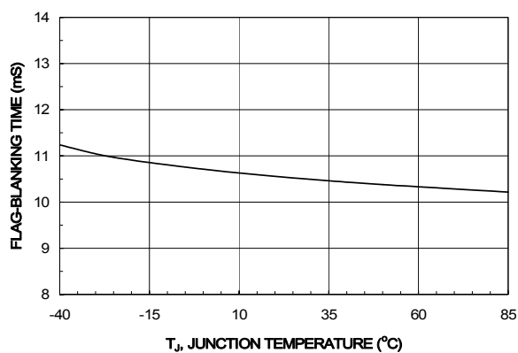
Figure 16. T_{BLANK} vs. Temperature
