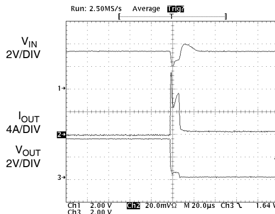
Figure 22. Short Circuit Response Time (Output Shorted to GND)
