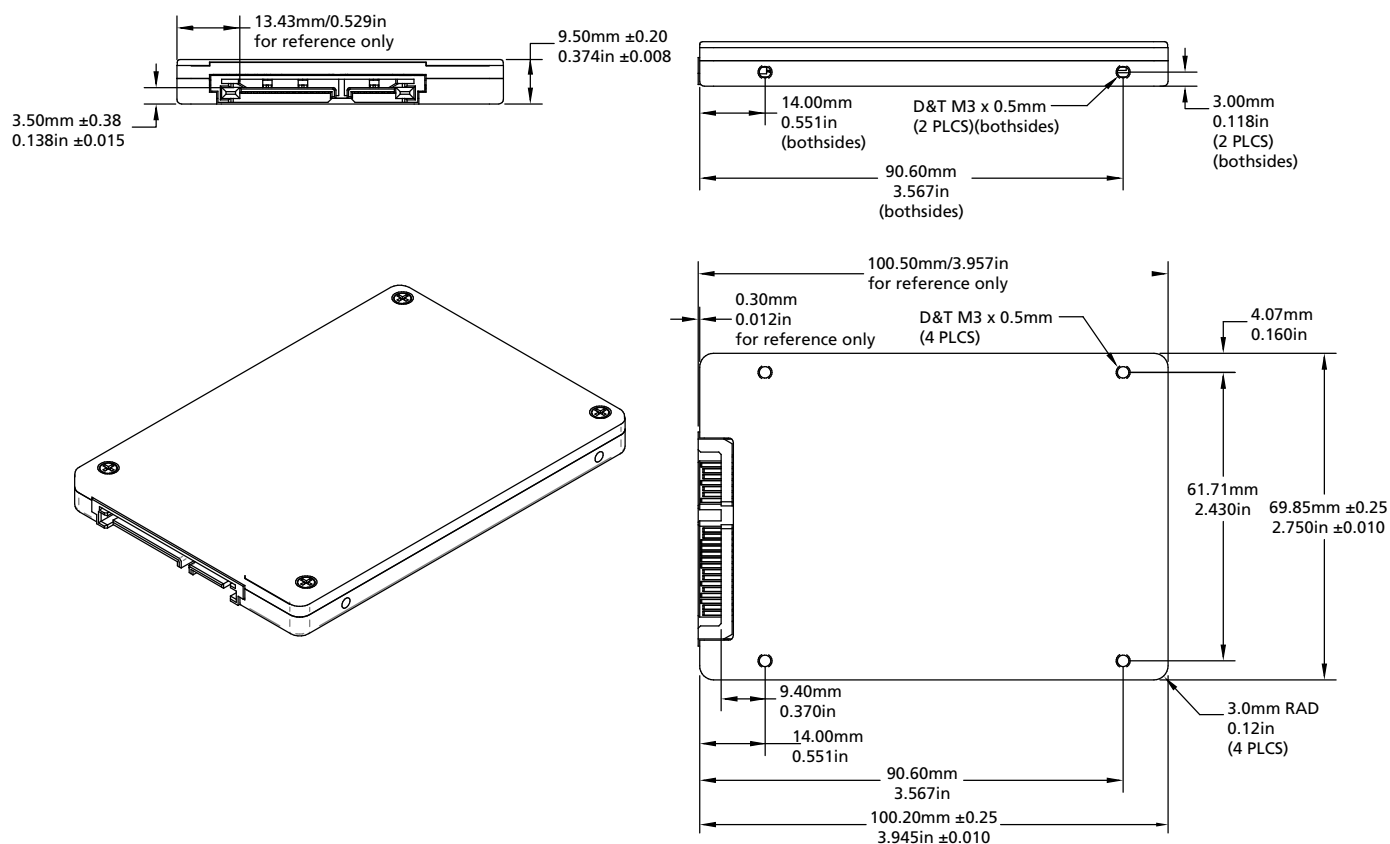
Figure 4: 2.5-Inch Package – 9.5mm
