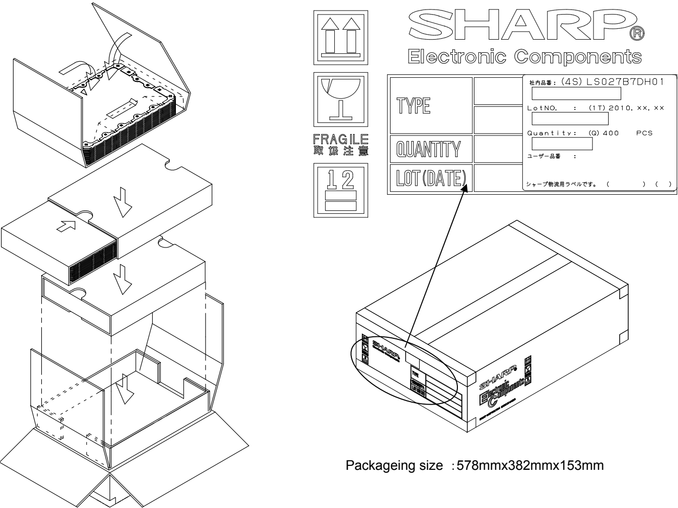
Figure 11-2 Packaging Condition
