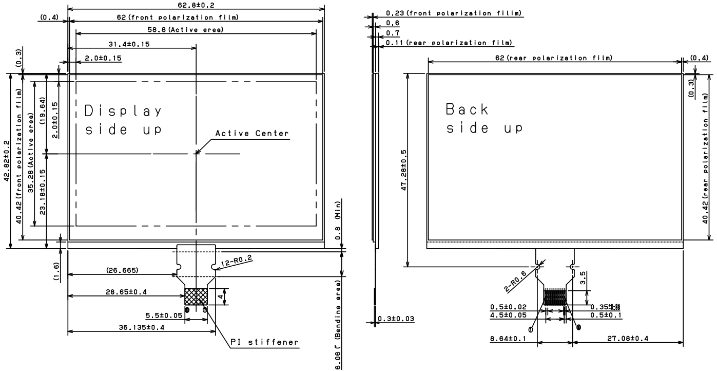
Figure 8-1 2.7" WQVGA Monochrome Outline Dimension
