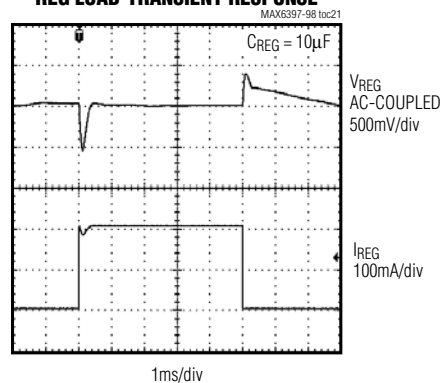
REG LOAD-TRANSIENT RESPONSE
