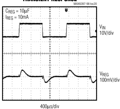
TRANSIENT RESPONSE
