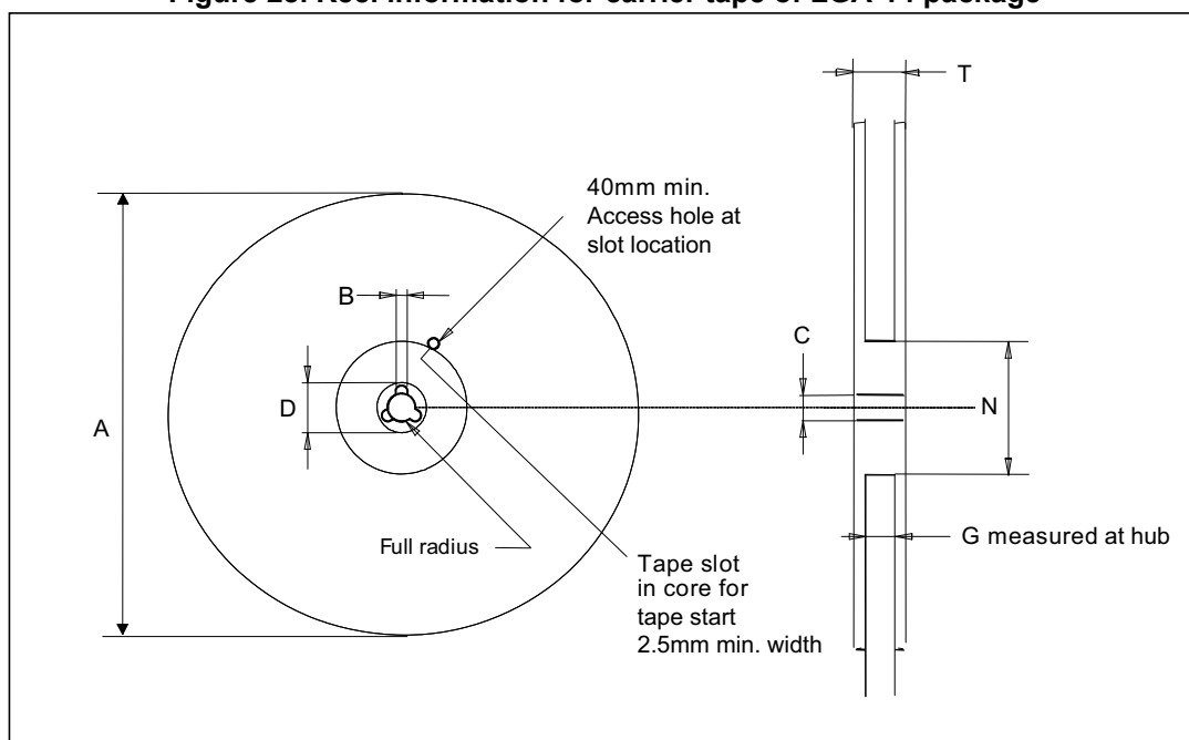
Figure 28. Reel information for carrier tape of LGA-14 package
