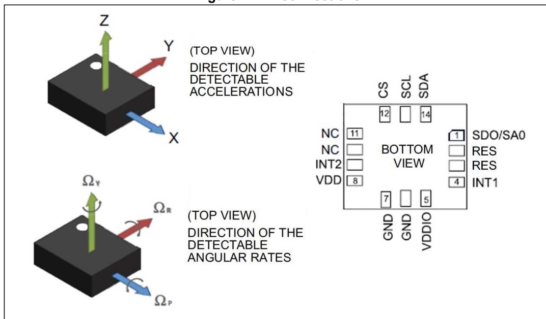
Figure 1. Pin connections
