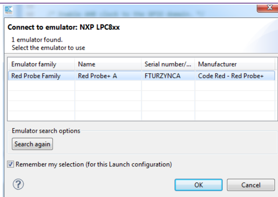
Figure 4.9. Attached probes – Red Probe+
