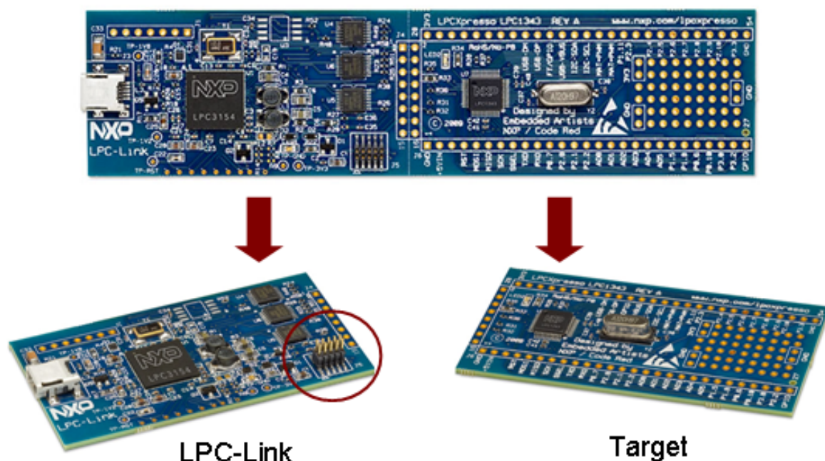
Figure 1.1. LPCXpresso development board
