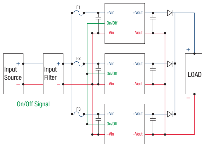
Figure 4. Redundant Parallel Connections
