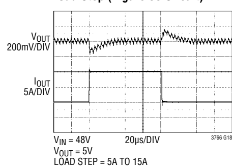
Load Step (Figure 39 Circuit)
