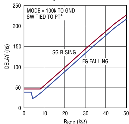
SGD Delay vs Resistance
