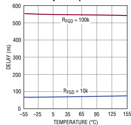
FGD Delay vs Temperature
