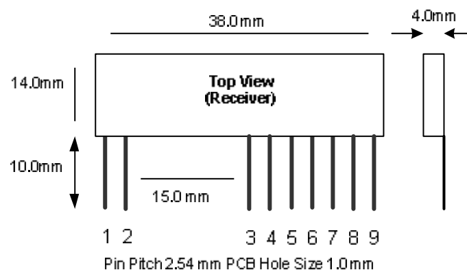
Figure 4 Physical Dimensions
