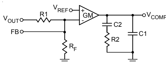
Figure 7. Compensation Loop
