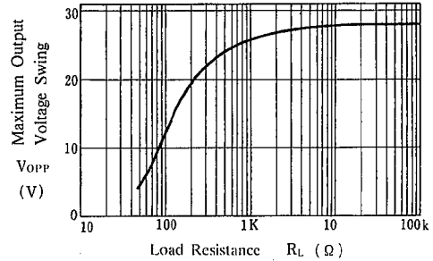
Maximum Output Voltage Swing vs. Load Resistance
