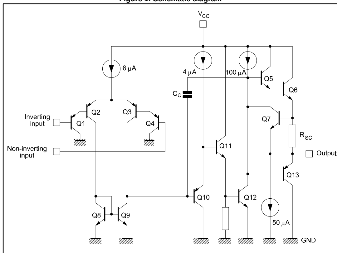
Figure 1: Schematic diagram
