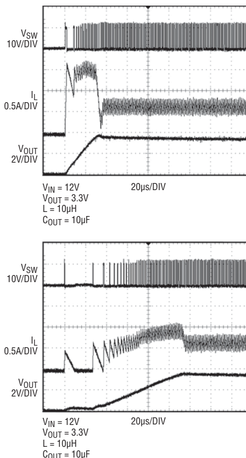
Figure 7. To Soft-Start the LT3493, Add a Resistor and Capacitor to the \overline{\text{SHDN}} Pin. V_{\text{IN}} = 12\text{V} , V_{\text{OUT}} = 3.3\text{V} , C_{\text{OUT}} = 10\mu\text{F} , R_{\text{LOAD}} = 5\Omega
