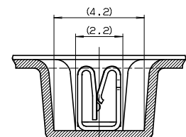
SECT. B-B
