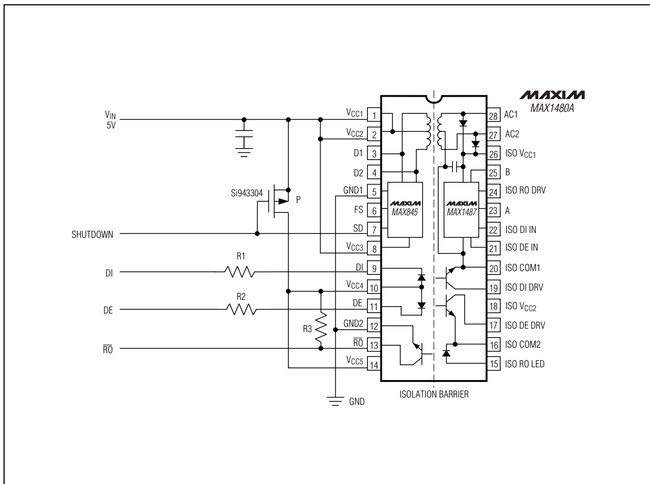
Figure 3. MAX1480A Low-Power Shutdown Mode
