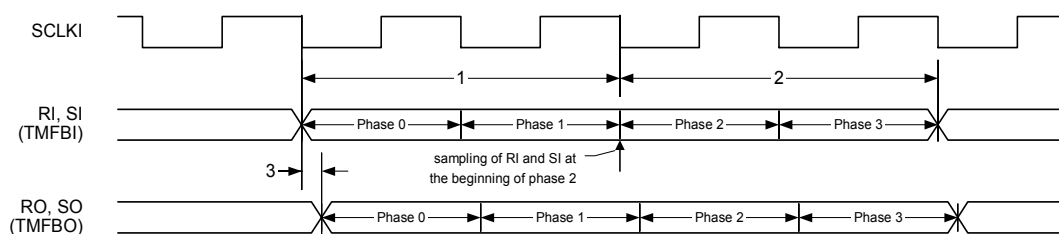
PCM Signal Timing and Frame Alignment
