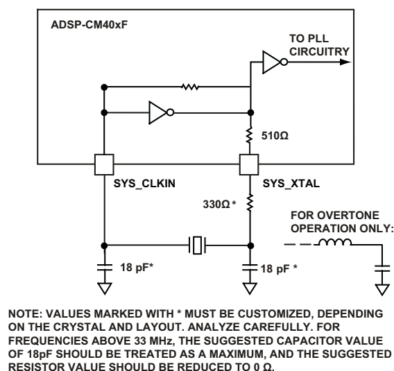
Figure 8. External Crystal Connection
