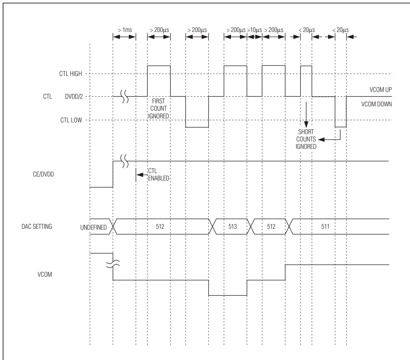
Figure 10. VCOM Adjustment
