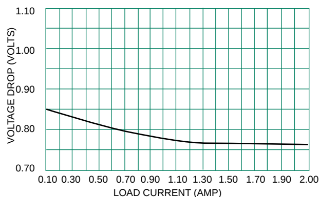
TYPICAL VOLTAGE DROP VS LOAD CURRENT OF KA/LA SERIES WITHOUT HEATSINK FIGURE 4
