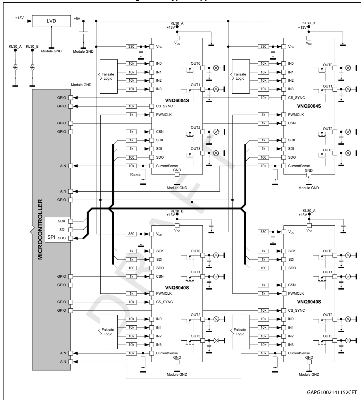
Figure 24. Typical application
