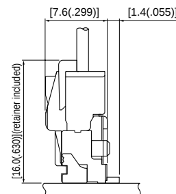
PA Receptacle + PA Header (Retainer mountable type)
