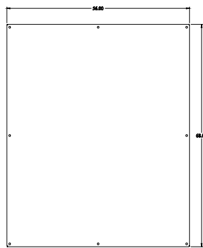
INNER PANEL
