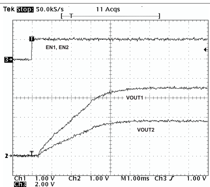
Figure 40. Ratiometric Start-Up Using Coupled SS/TR Pins
