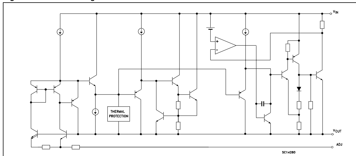
Figure 1: Schematic Diagram
