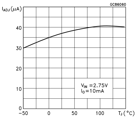
Figure 12: Adjust Pin Current vs Temperature
