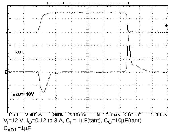
Figure 24: Load Transient
