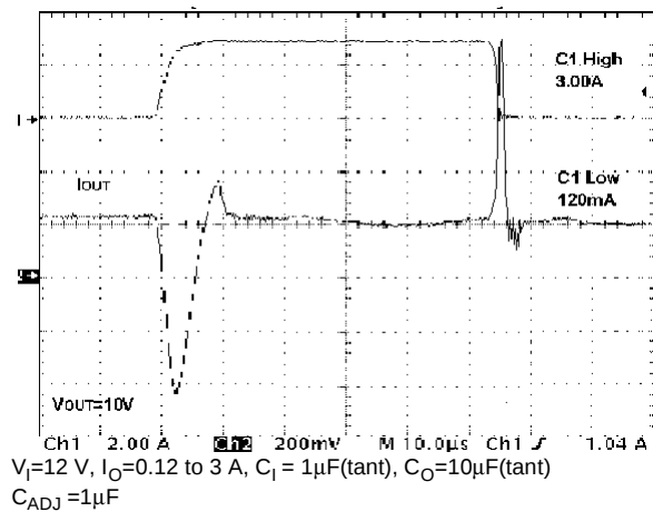
Figure 23: Load Transient
