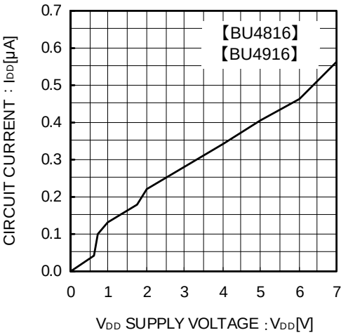
Fig.3 Circuit Current
