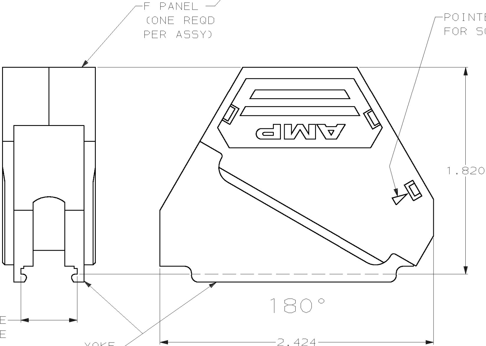
TYPICAL CABLE SUPPORT GATE (ASSORTMENT SUPPLIED WITH CABLE CLAMP ASSEMBLIES).
