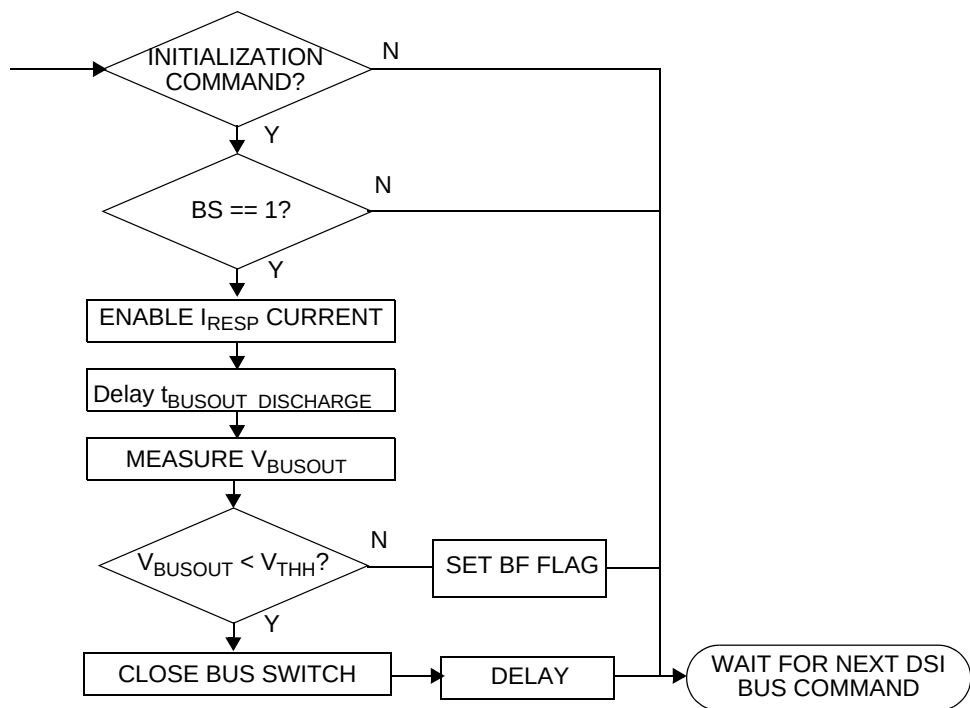
Figure 22. Initialization Sequence
