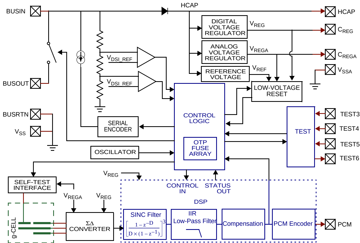
Figure 3. Block Diagram
