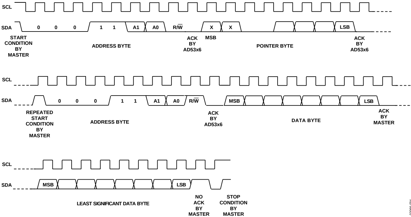
Figure 34. Readback Sequence
