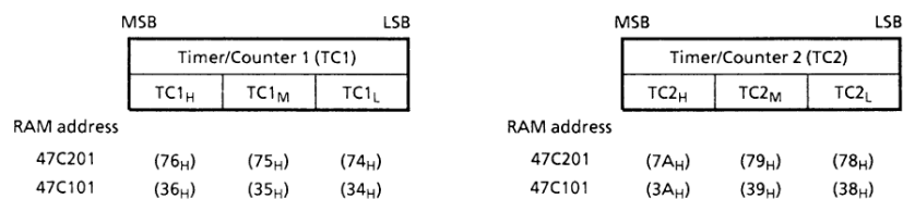
Figure 2-9. Count Registers of the Timer/Counters (TC1, TC2)
