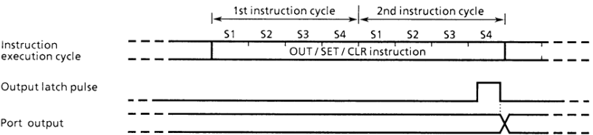
Figure 3-2. Output Timing
