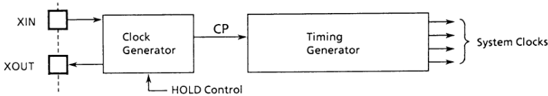
Figure 2-14. Clock Generator and Timing Generator
