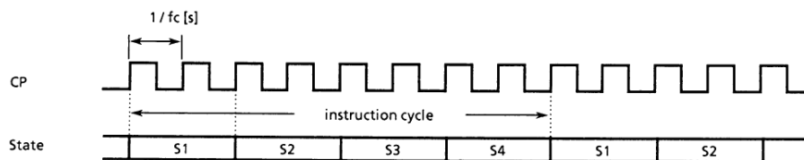
Figure 2-17. Instruction Cycle
