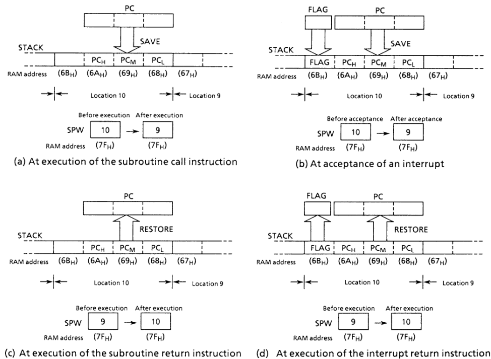
Figure 2-8. Accessing Stack (Save/Restore) at the 47C201
