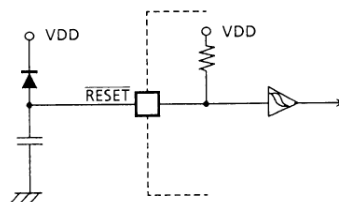
Figure 2-23. Simplified Power-On-Reset
