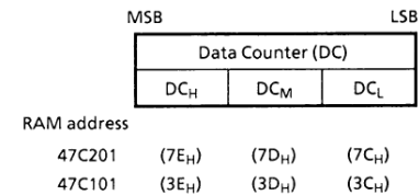
Figure 2-7. Data Counter
