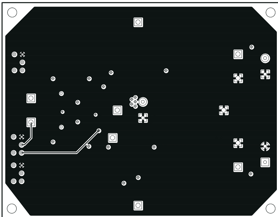
Figure 8-5. Internal Layer 1
