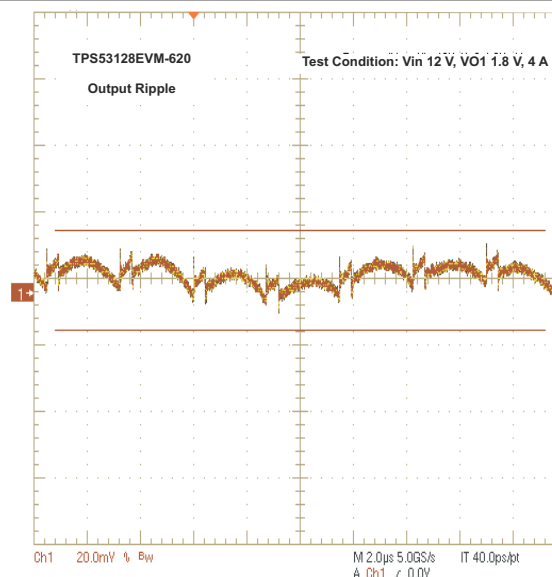
Figure 7-6. Output Voltage Ripple
