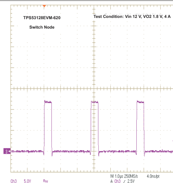
Figure 7-8. Switching Waveform
