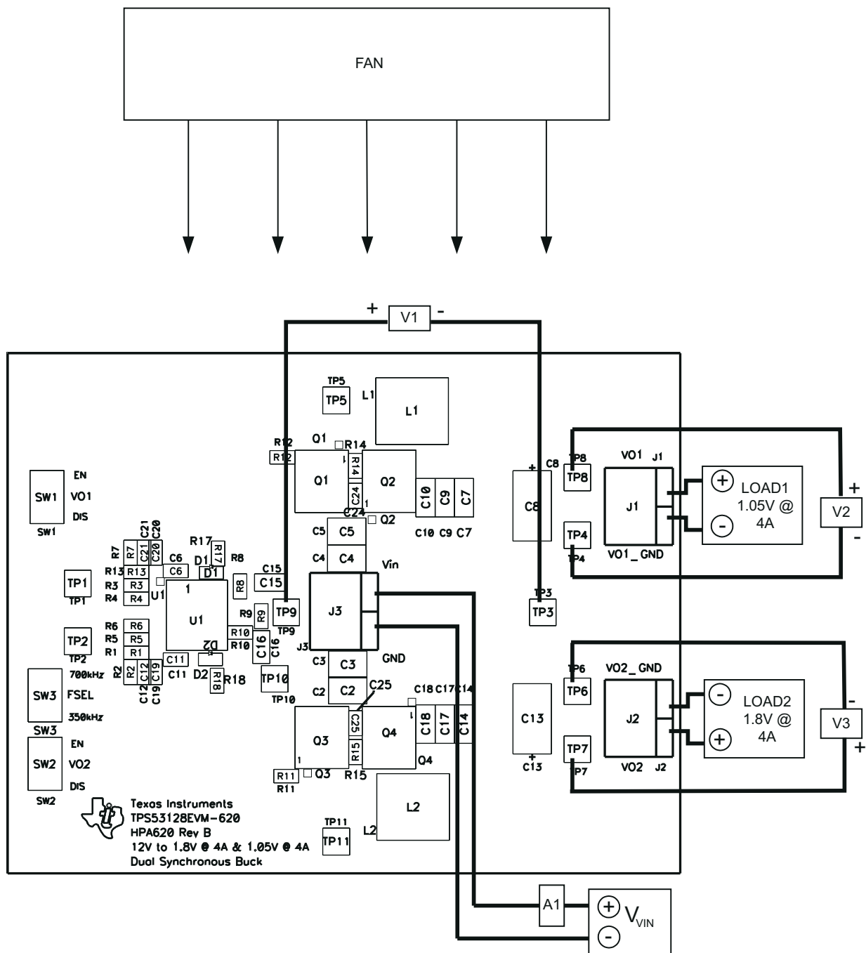
Figure 5-1. TPS53128EVM-620 Recommended Test Setup
