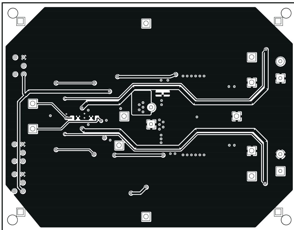
Figure 8-4. Bottom Layer
