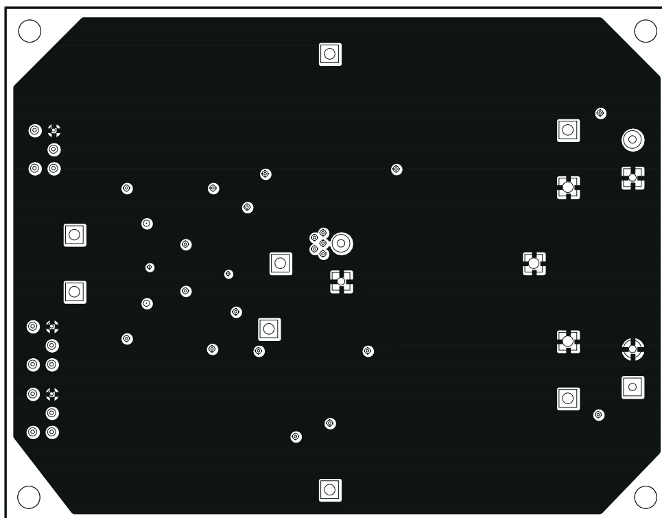
Figure 8-6. Internal Layer 2
