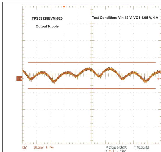
Figure 7-5. Output Voltage Ripple
