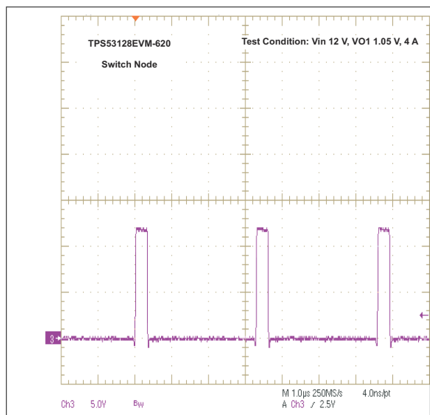
Figure 7-7. Switching Waveform
