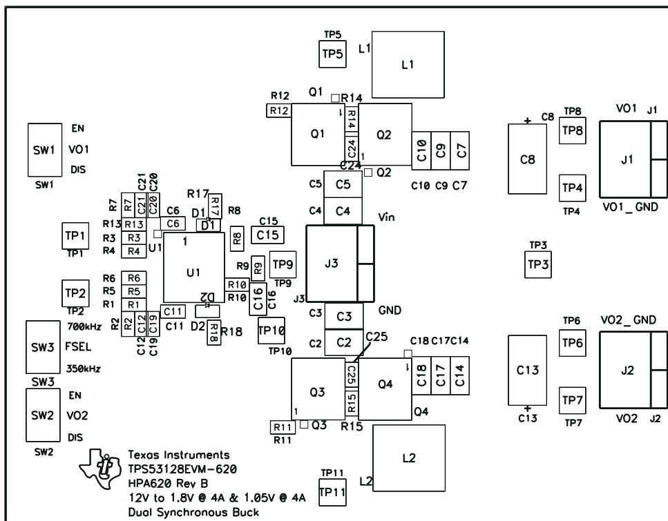
Figure 8-1. Top Assembly
