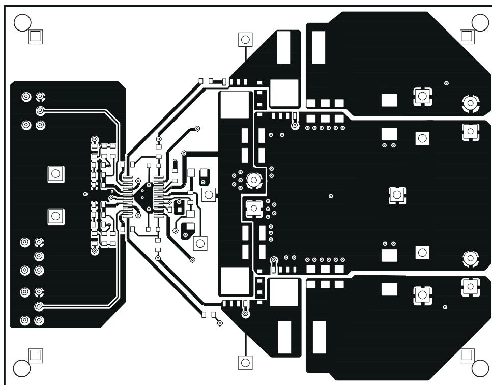
Figure 8-3. Top Layer
