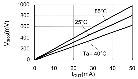
S-817A50A/S-817B50A
