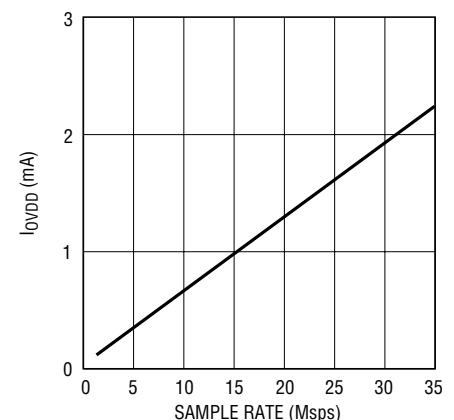
LTC2236: I_{OVPD} vs Sample Rate, 5\text{MHz} Sine Wave Input, -1\text{dB} , O_{VDD} = 1.8\text{V}
