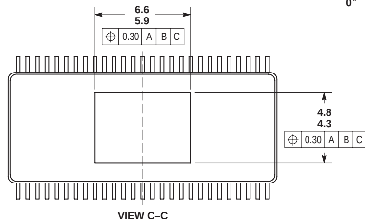
VIEW C-C
