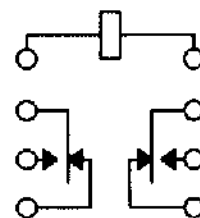
TERMINAL VIEW
