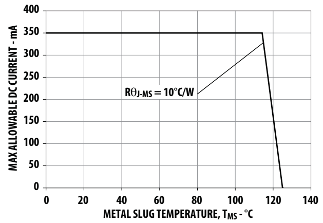
Figure 11. Maximum Forward Current vs. Metal Slug Temperature. Derated based on T_{JMAX} = 125^{\circ}\text{C} , R_{\theta MS} = 10^{\circ}\text{C/W} .
