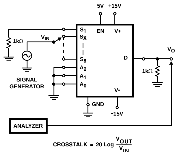
FIGURE 6. CROSSTALK
