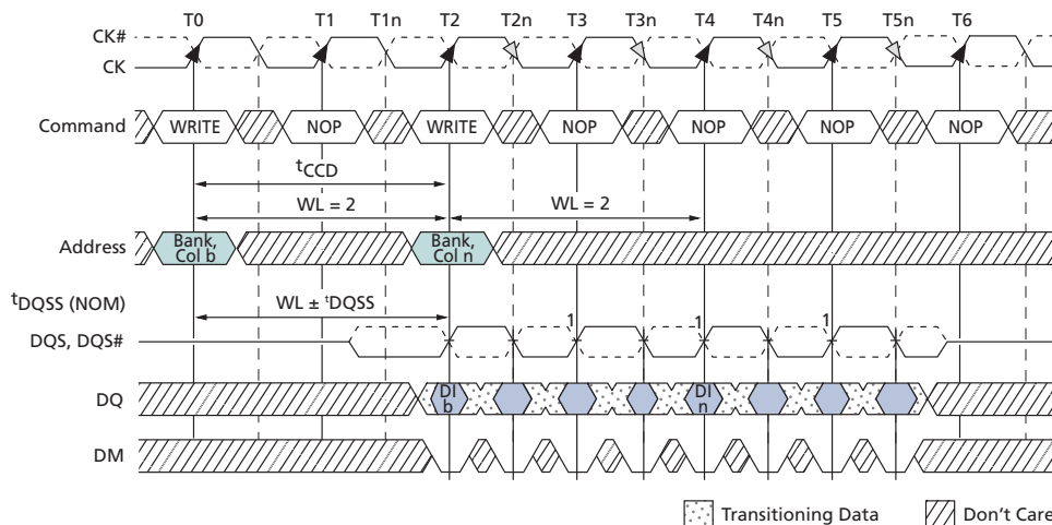
Figure 59: Consecutive WRITE-to-WRITE
