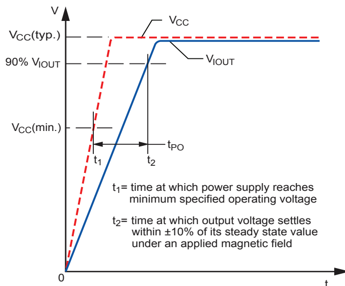
Figure 4: Power-On Time ( t_{PO} )
