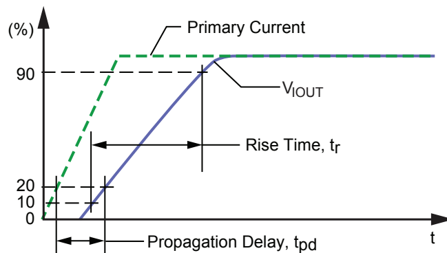
Figure 5: Rise Time ( t_r ) and Propagation Delay ( t_{pd} )
