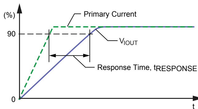
Figure 6: Response Time ( t_{RESPONSE} )
