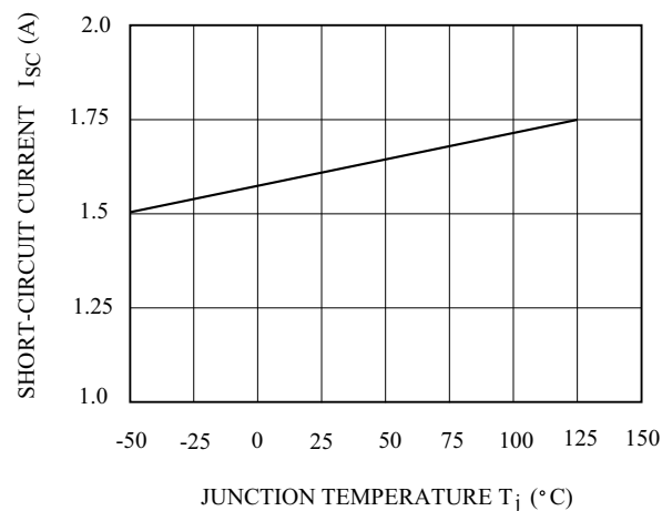
Fig.7 I_{SC} - T_j
