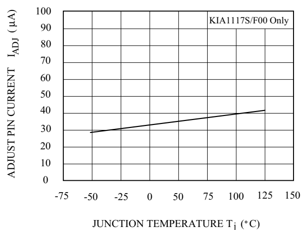
Fig.6 I_{ADJ} - T_j
