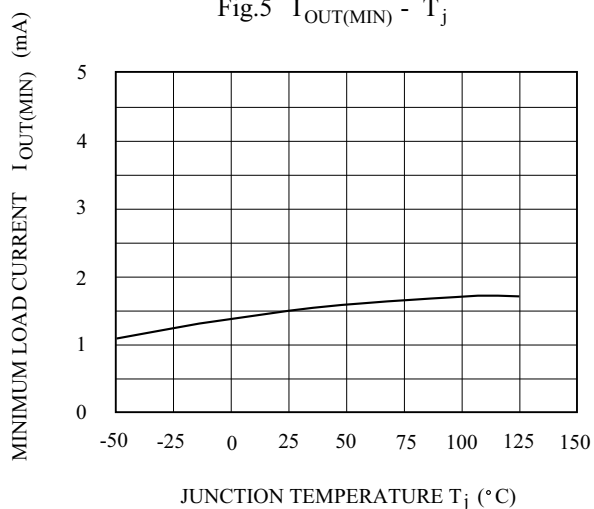
Fig.5 I_{OUT(MIN)} - T_j
