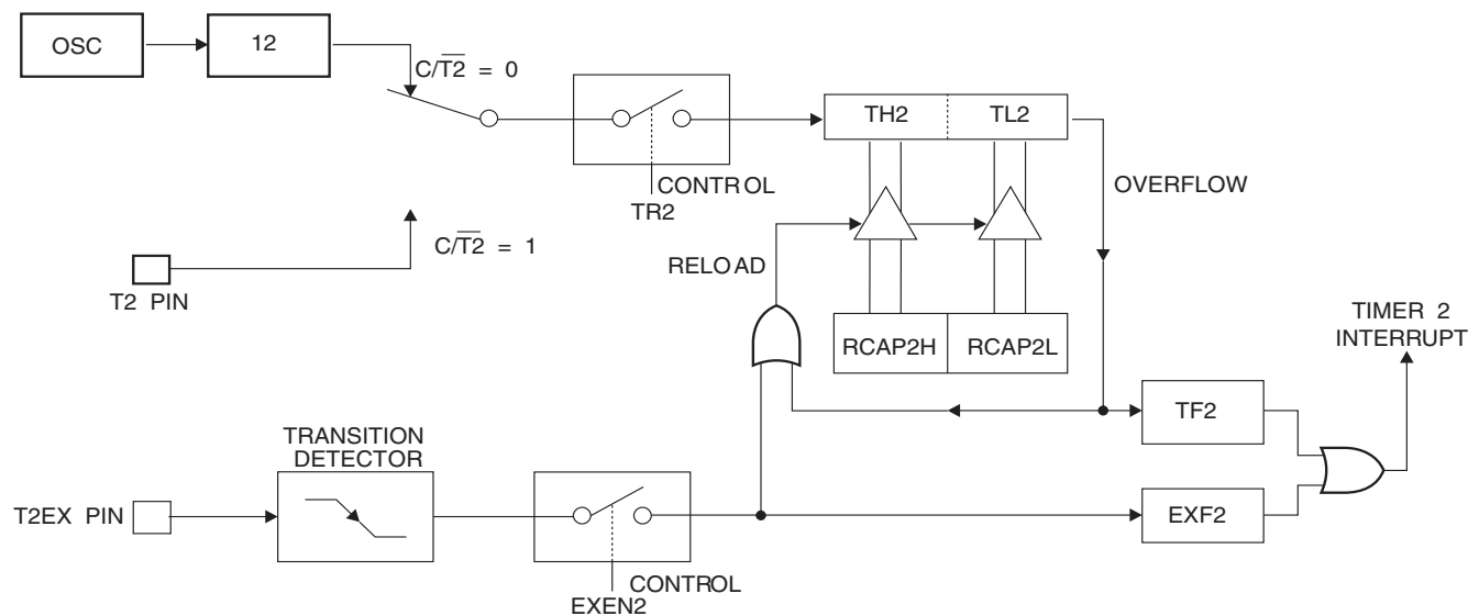
Figure 6. Timer 2 Auto Reload Mode (DCEN = 0)
